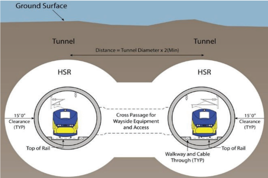
Figure 2. Illustrated cross-section showing the typical configuration of a dual-bore tunnel.
